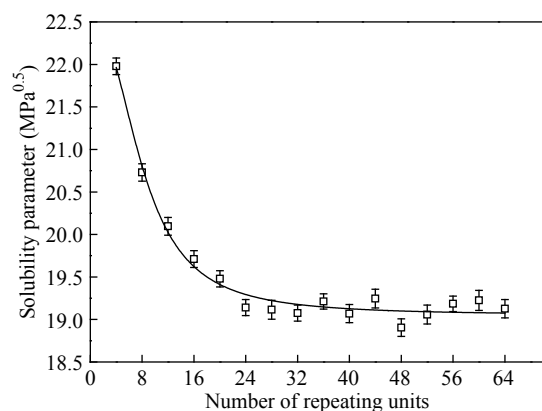
Fig. 3 Computed solubility parameter of PVC versus number of repeating units
